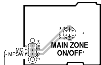
OPERATION (2) P.C.B. (Side A)
