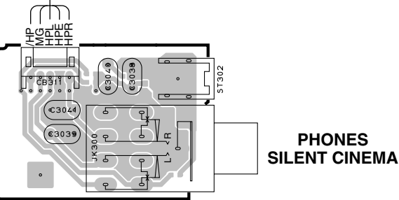
OPERATION (3) P.C.B. (Side A)
