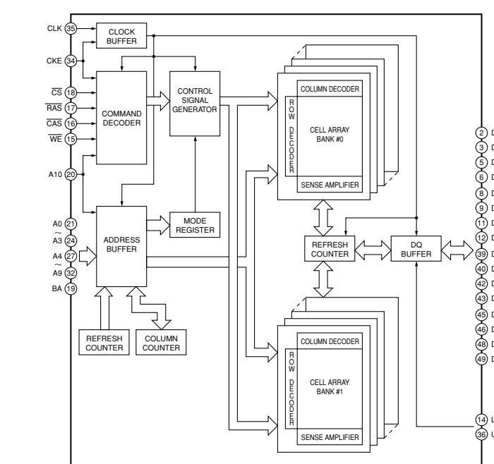
IC64 : W9816G6CH-7 512K x 2 banks x 16 bits SDRAM
