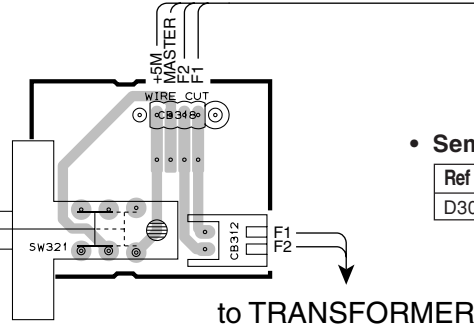
OPERATION (6) P.C.B. (Side A)
